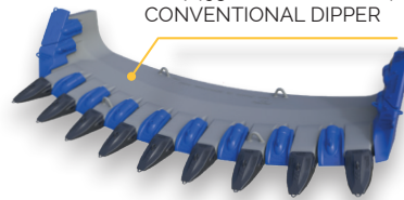
DIPPEREDGE (SQUARE EDGE) CAT7495 AND KOMATSU 4100A/XPB CONVENTIONAL DIPPER
