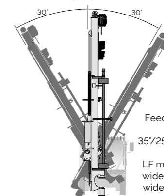
Feed swing angles - standard feed
