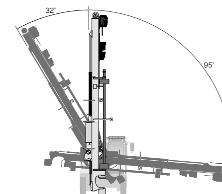
Feed swing angles - standard feed
