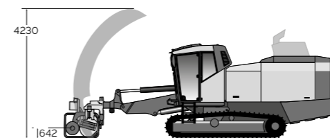
Toe-hole drilling (standard feed only)
