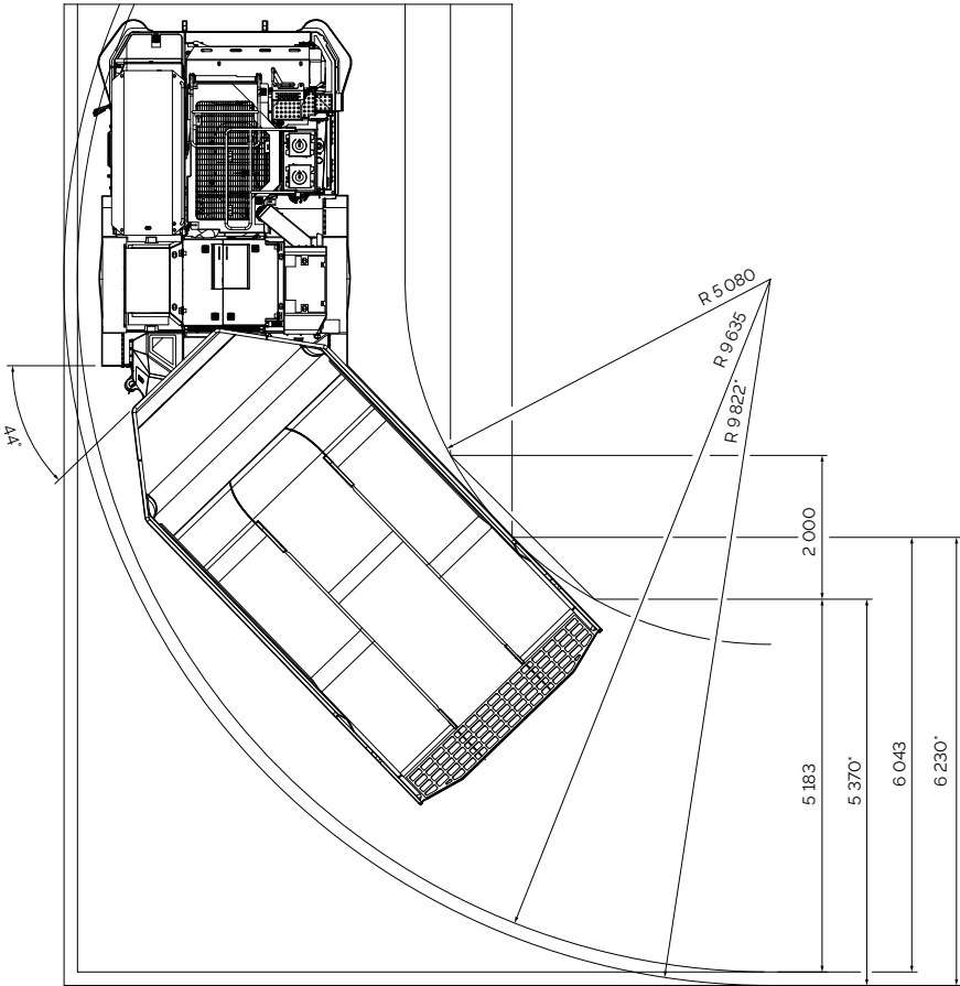
View showing box (1.6t/m³) * Refers to dimensions when batwings are included.
