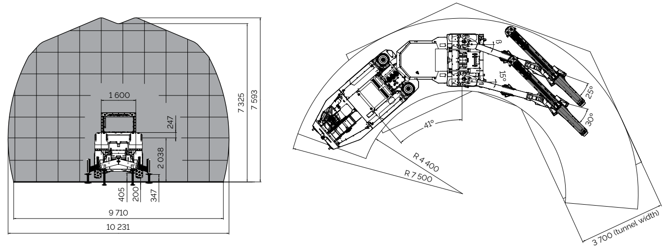
Boomer M20 S coverage area.
