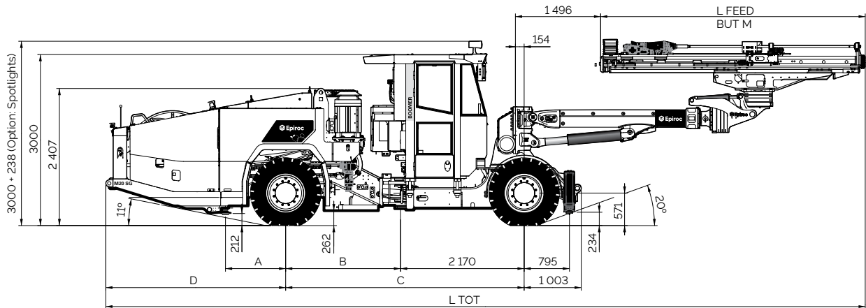
Boomer M20 SG equipped with COP MD20.
