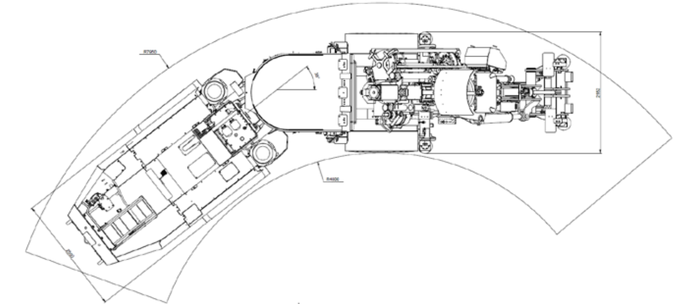
Illustration shows turning radius of Simba E60 S with 6-cylinder engine and E-tramming.
