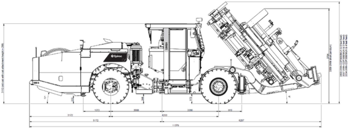
Illustration shows Simba E60 S in right side view with 6-cylinder engine and E-tramming.
