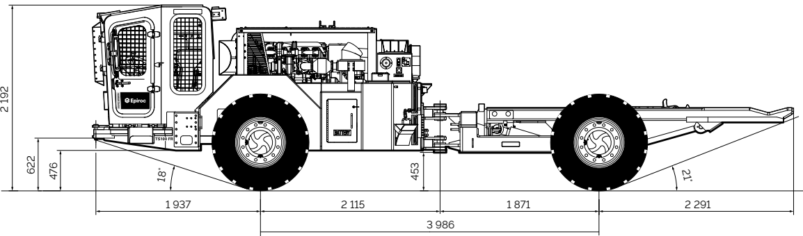
Left side view of Terrah TS100 FR
