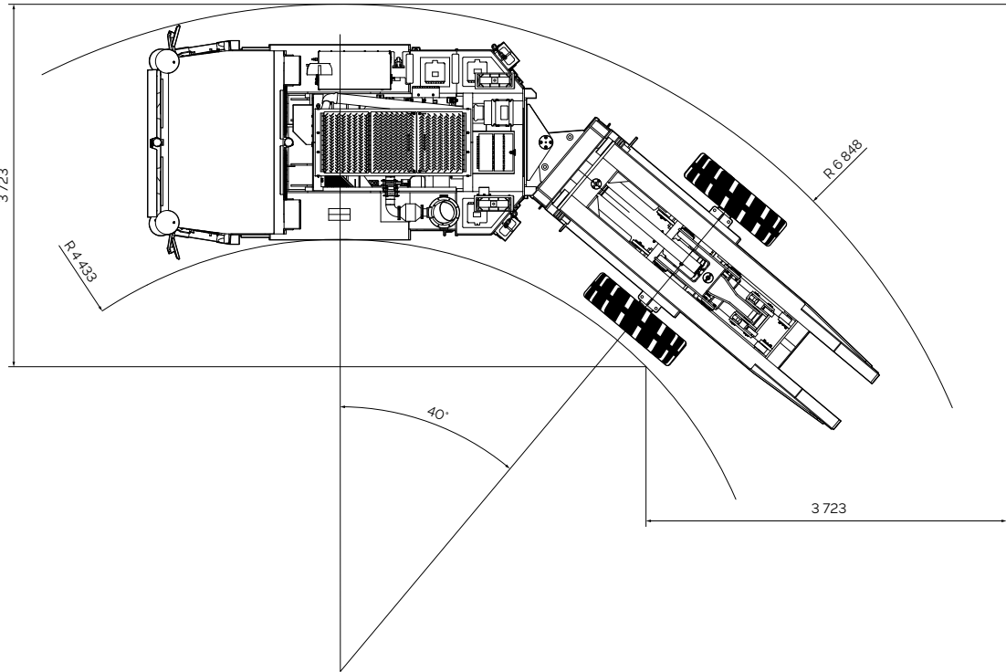
Turning radius of Terrah TS100 FR
