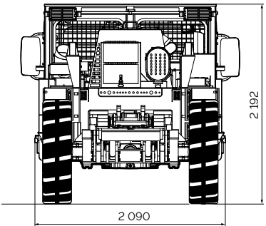
Rear view of Terrah TS100 FR.
