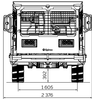
Front view of Terrah TS100 FR.
